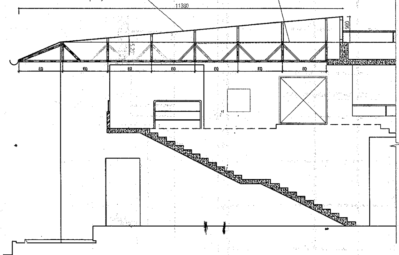
Section through courtyard
