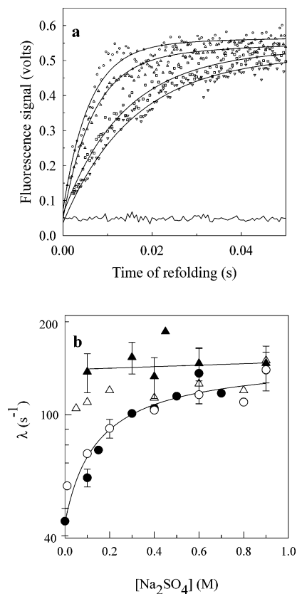
FIGURE 6: Core compaction is the rate-limiting step in the folding of barstar. (a) Refolding traces in 0.1 M Na 2 SO 4 at pH 7 are shown when refolding is initiated from different initial conditions. The different symbols represent refolding initiated from the pH 12 unfolded D form ( \nabla ), the 0.1 M Na 2 SO 4 , pH 12 P form ( \square ), the 0.6 M Na 2 SO 4 , pH 12 ICC form ( \Delta ), and the 1 M Na 2 SO 4 , pH 12 B form ( \circ ). (b) Refolding rates (fast phase) of the pH 12 unfolded D form ( \bullet ), 1 M Na 2 SO 4 , pH 12 B form ( \blacktriangle ), 0.1 M Na 2 SO 4 , pH 12 P form ( \circ ), and 0.6 M Na 2 SO 4 , pH 12 ICC form ( \Delta ) when refolded in different concentrations of Na 2 SO 4 in the range of 0–1 M, at pH 7. The values represent the means, and the error bars represent the standard deviations from three separate experiments. The line through the data is a mere guide to the eye and does not represent any functional dependence of the observed rates on Na 2 SO 4 concentration.
